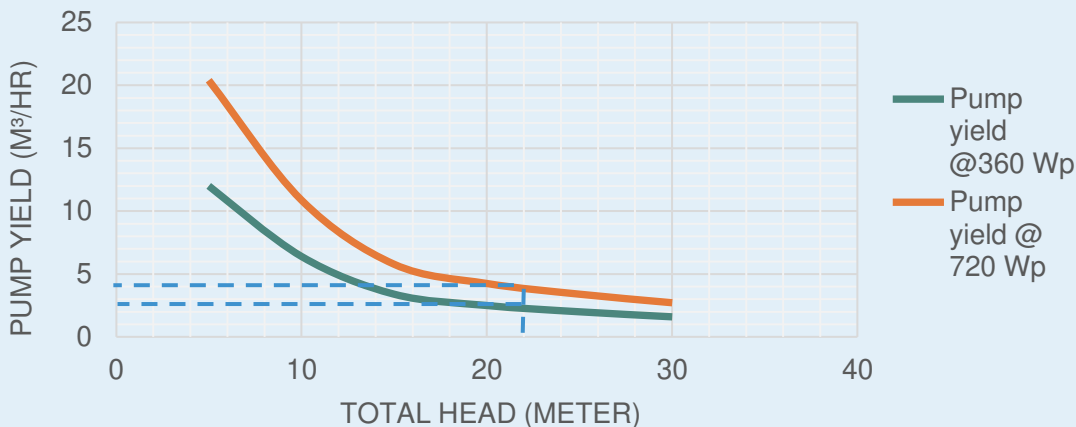
Pump curve
