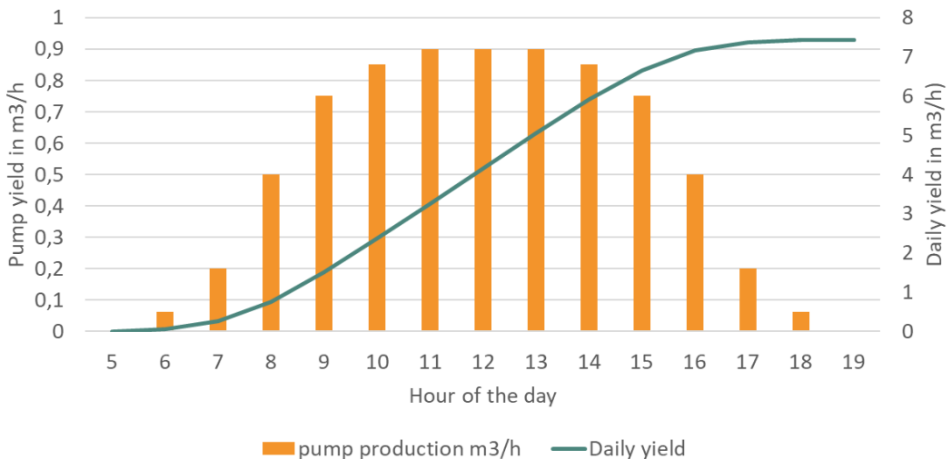
Pump yield (in m 3 /h) per hour and per day
